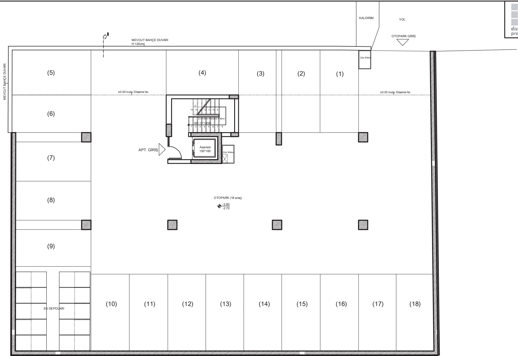
BODRUM KAT PLANI Alan:400m 2
